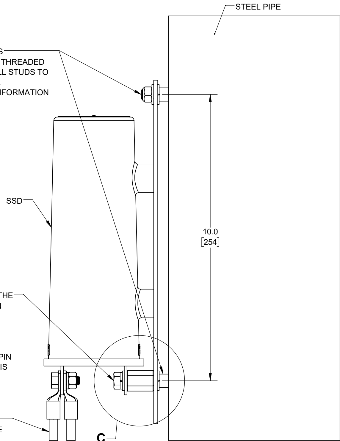
DETAIL B SCALE 1 : 2
