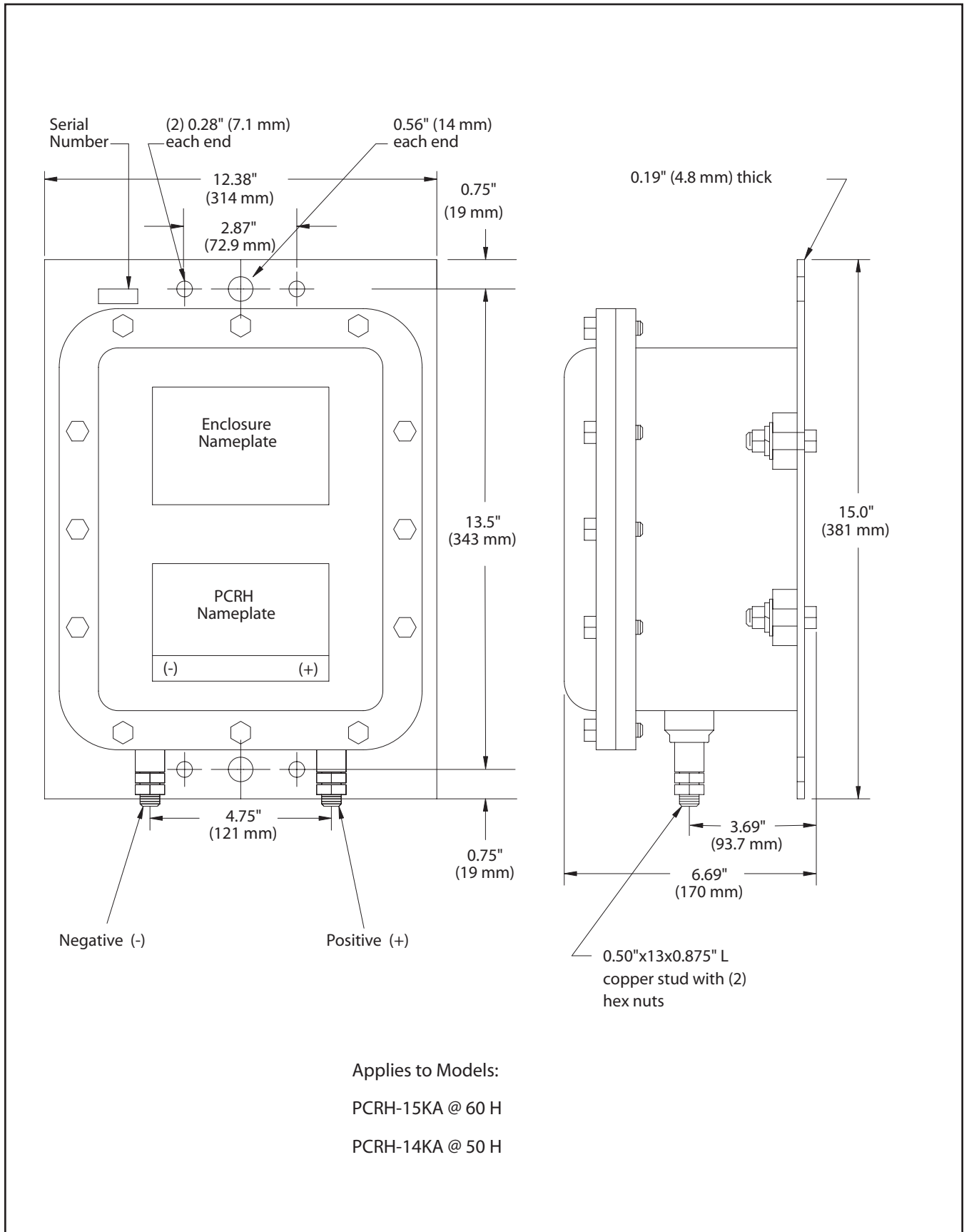
FIGURE 1B PCRH Outline Dimensions
