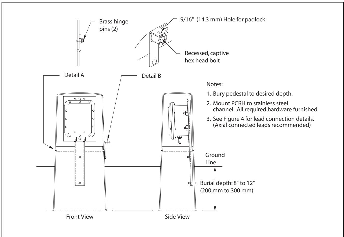
FIGURE 5 PCRH Mounted in Pedestal Enclosure
