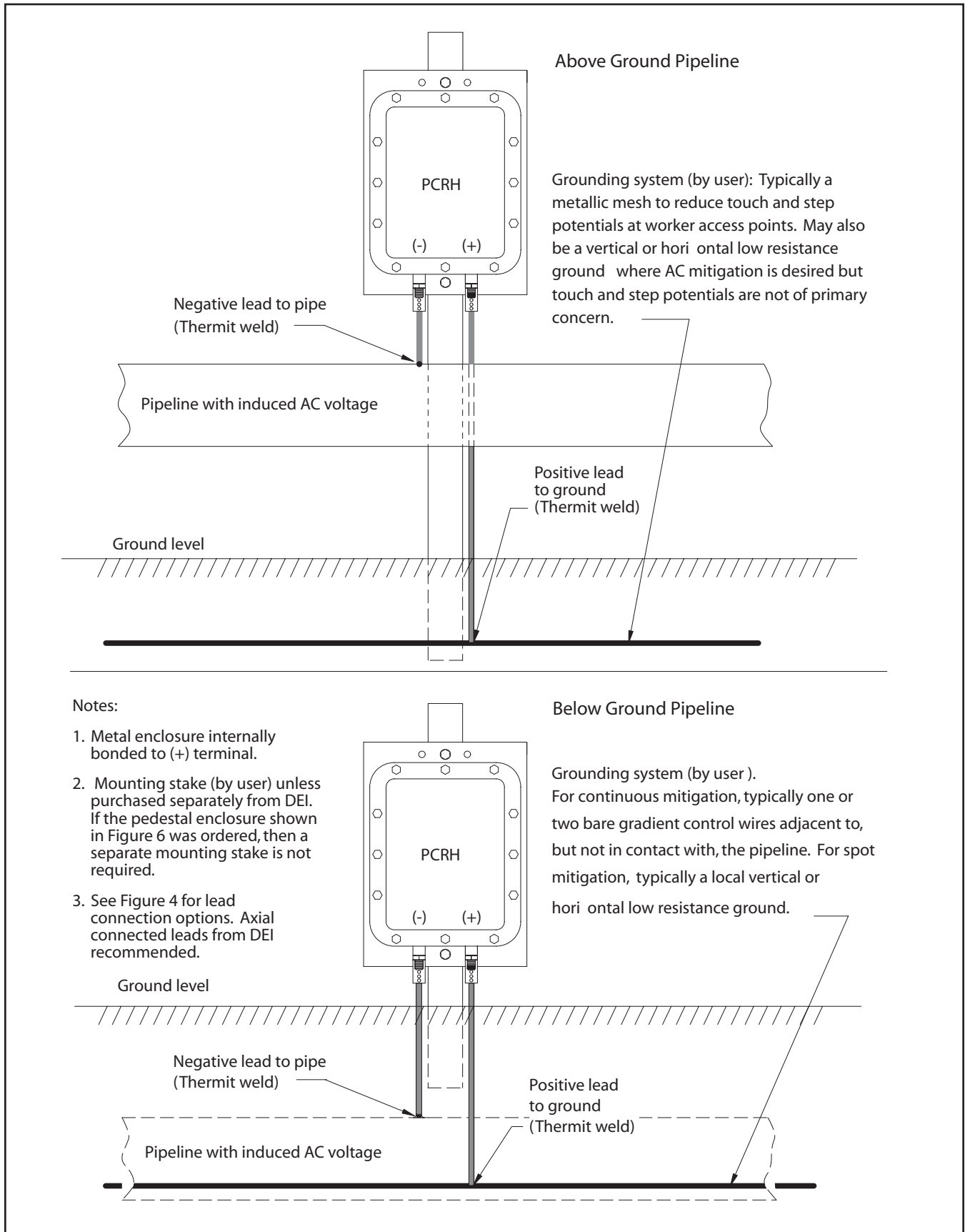
FIGURE 6 Typical Installation for AC Voltage Mitigation
