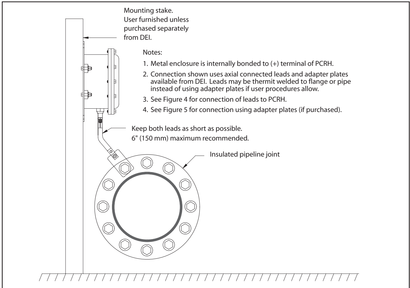
FIGURE 3 PCRH Lead Connection Options
