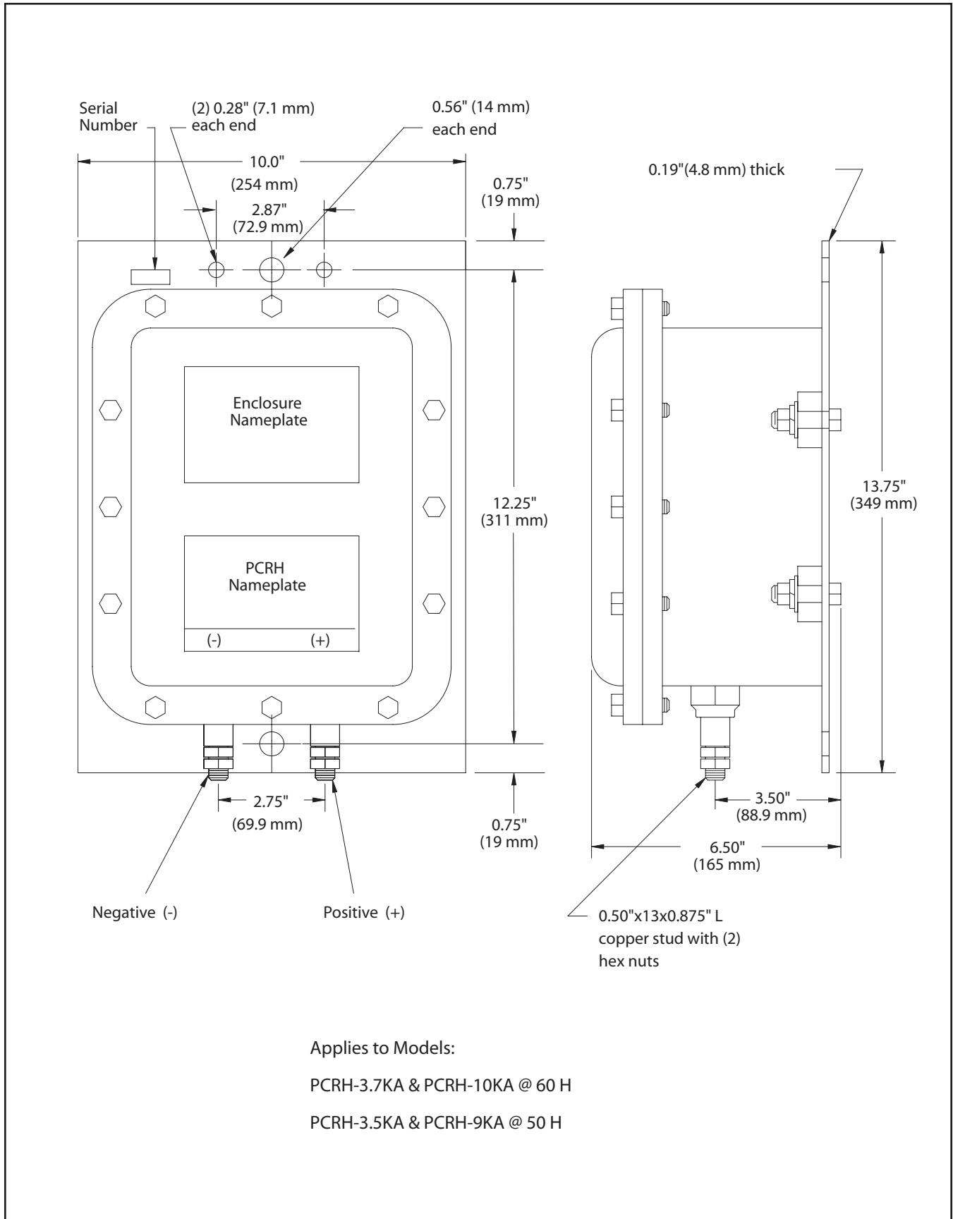
FIGURE 1A PCRH Outline Dimensions
