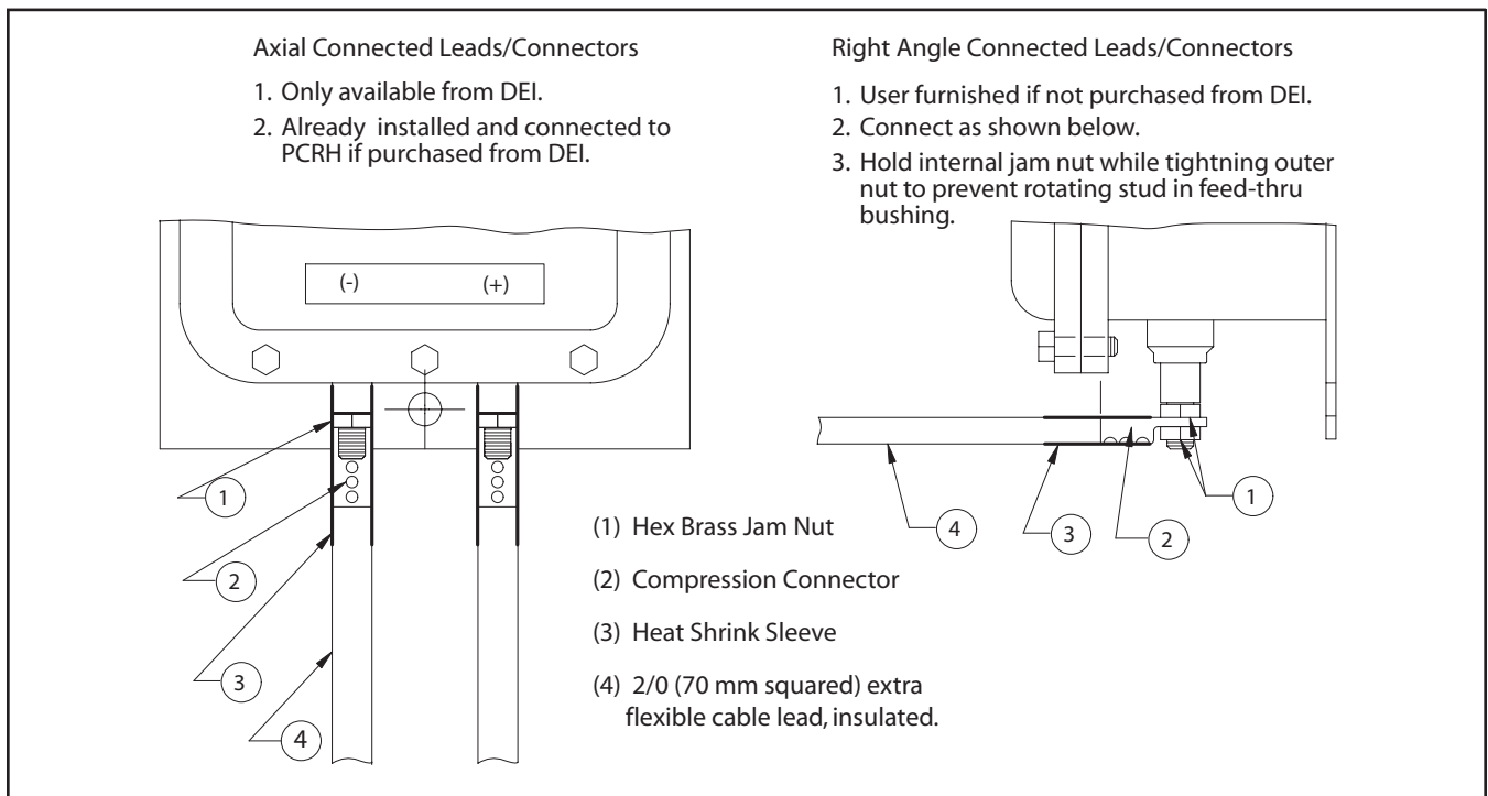
FIGURE 3 PCRH Lead Connection Options
