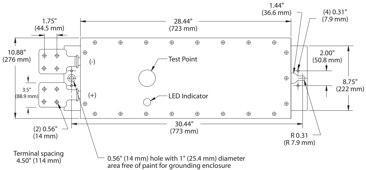
FIGURE 7B ISP Outline Dimensions
