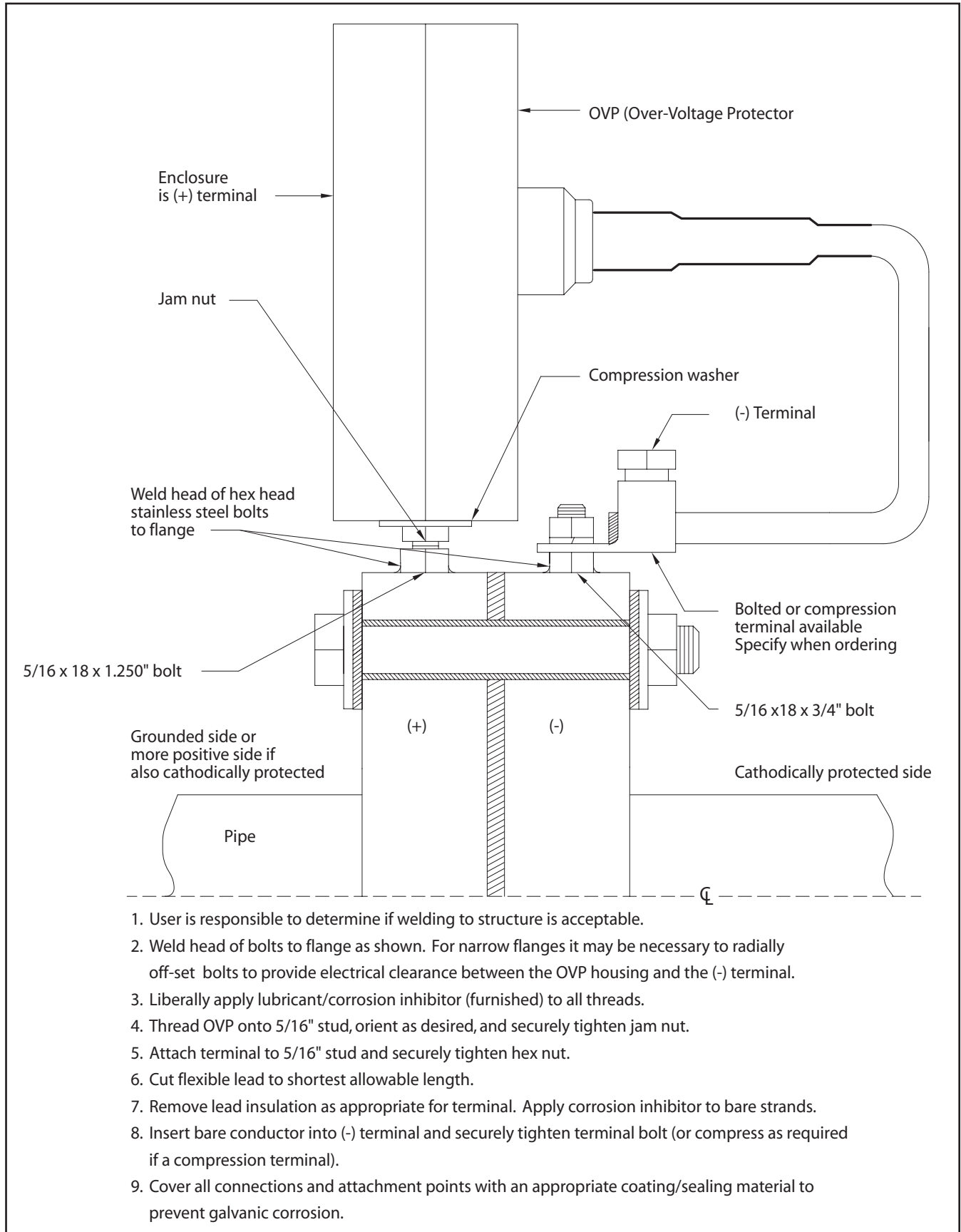
FIGURE 1 Flange Mount Using Welded Hex Bolts Using FMWHB Mounting Kit
